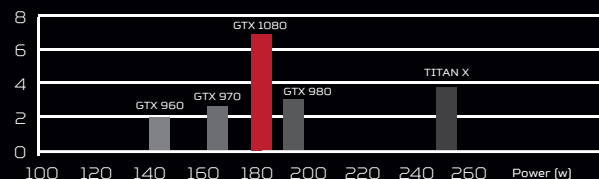
2X PERF AND 3X EFFICIENCY VS. TITAN X
